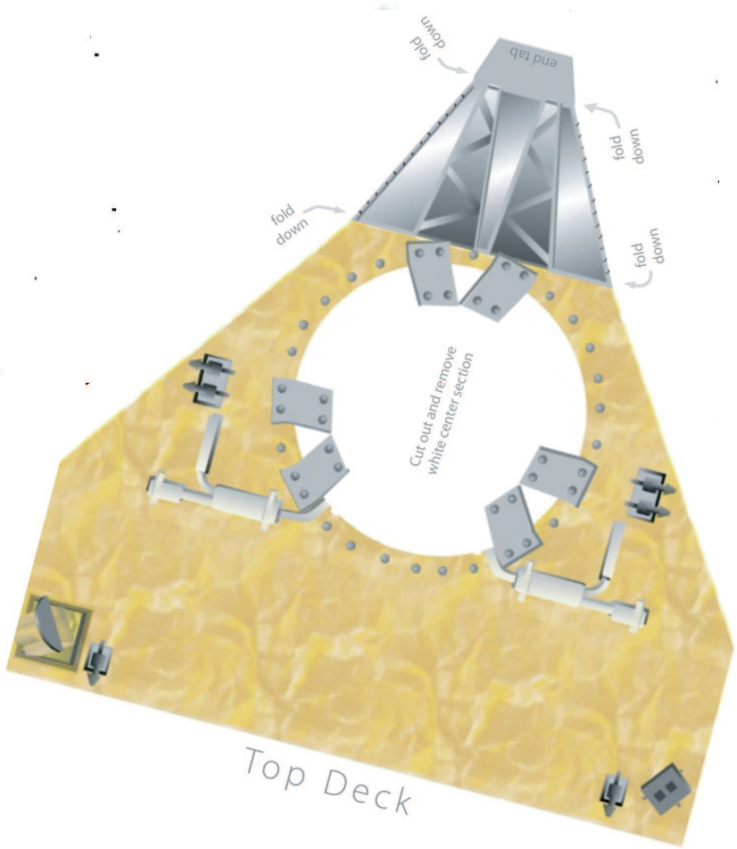
High Gain Antenna Top – HGA
